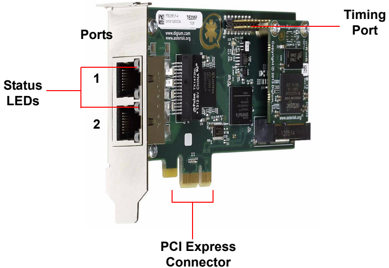
Figure 4: TE235B Card
