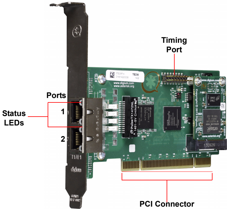
Figure 5: TE236B Card
