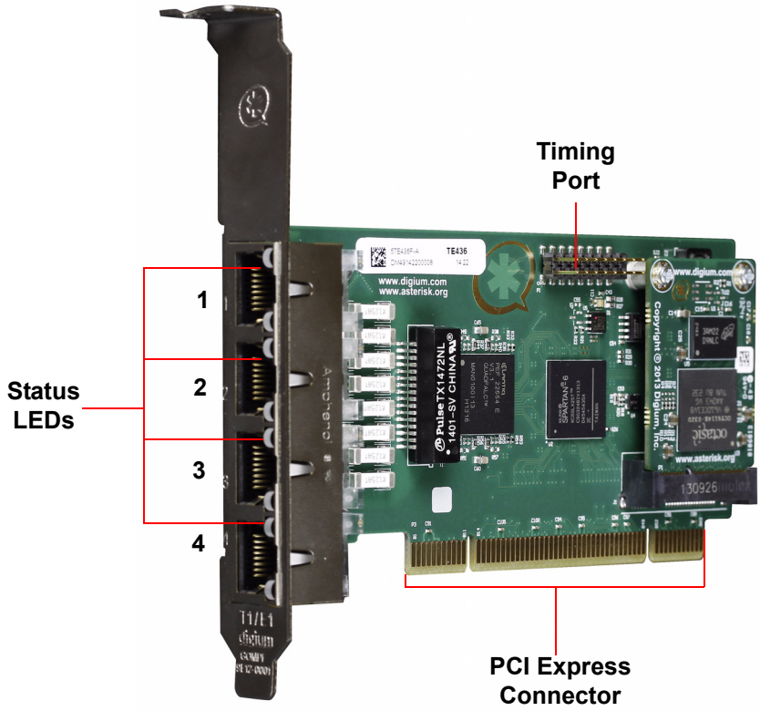
Figure 5: TE436B Card
