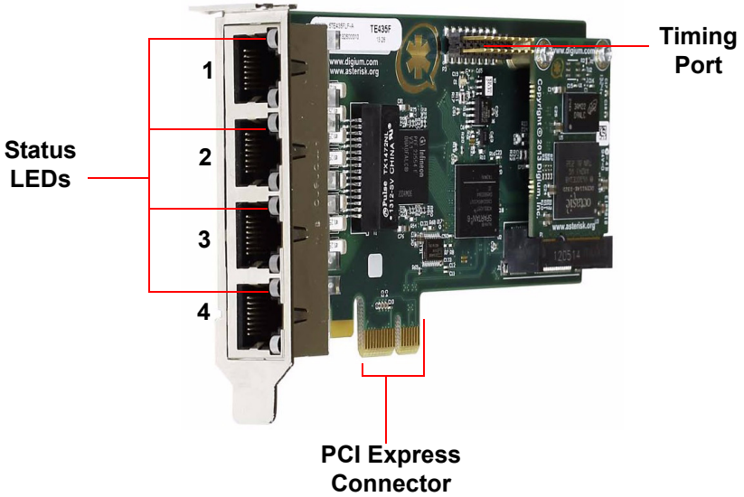
Figure 4: TE435B Card
